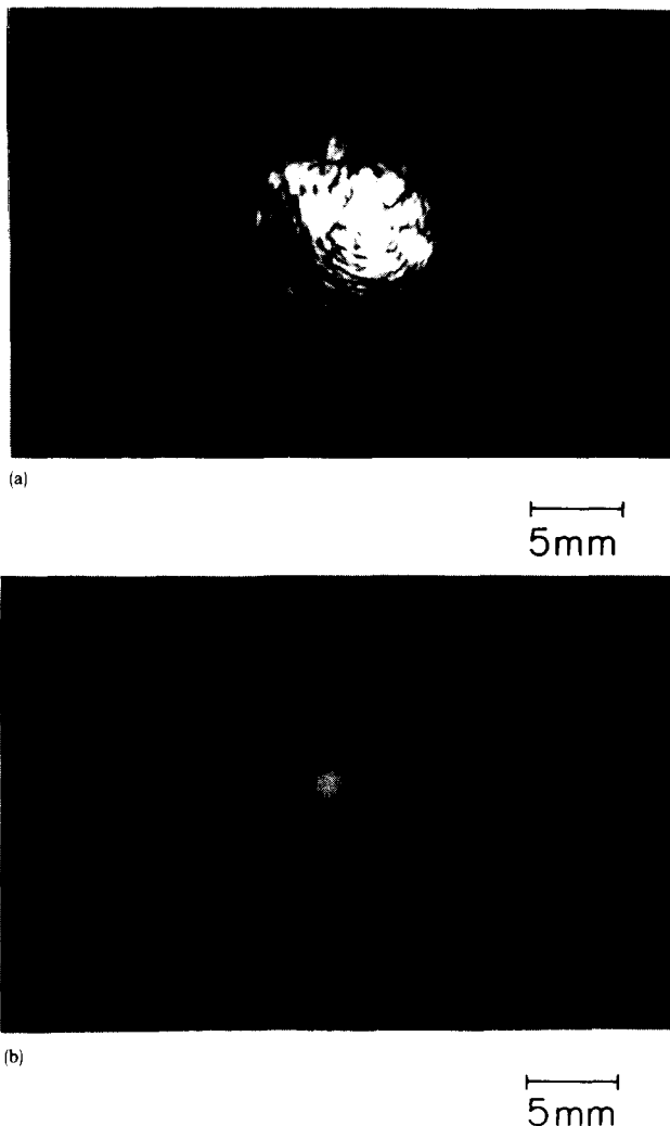
FIG. 2. (a) Photograph of the output of regular laser (i.e., crystal replaced by high reflectivity dielectric mirror) containing an intracavity distortion. The distance from the output mirror M_1 is 1 m. The laser intensity is 1 mW, obtained at 38 A laser tube current. (b) The output of the passive phase conjugate resonator laser containing the intracavity distortion. The distance from the output mirror M_1 is one meter. The laser intensity here is 3 mW, obtained at only 21 A laser tube current. The power output at 38 A is 500 mW.
